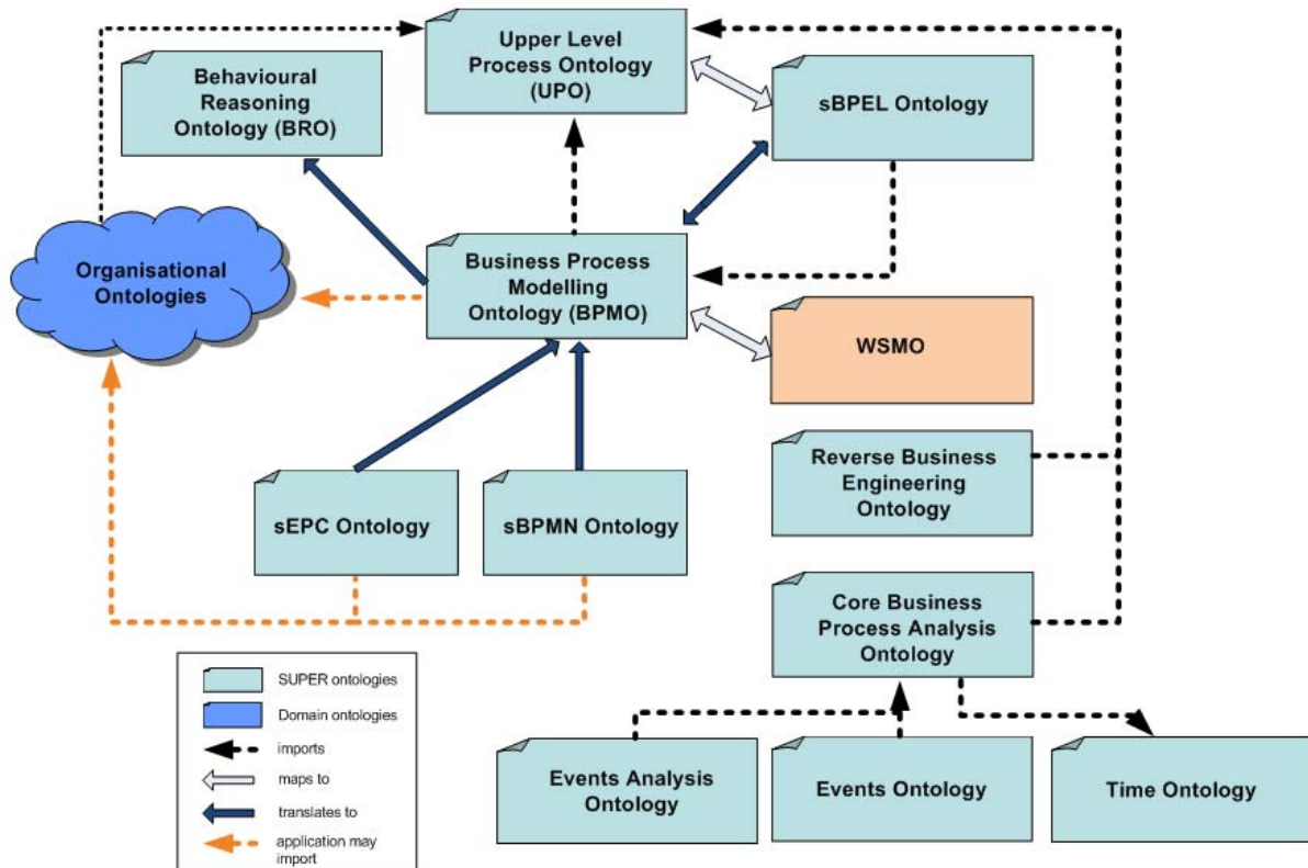
Figure A – SUPER Process Ontology Stack
