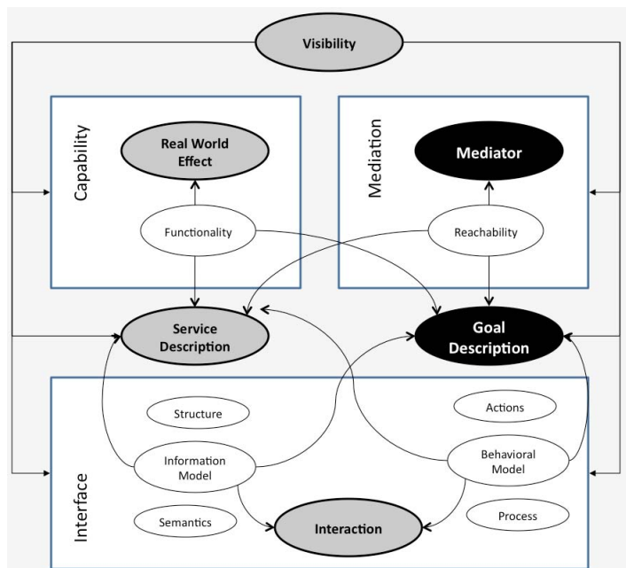
Figure B – Extensions (shown in black) to the OASIS SOA Reference Model
