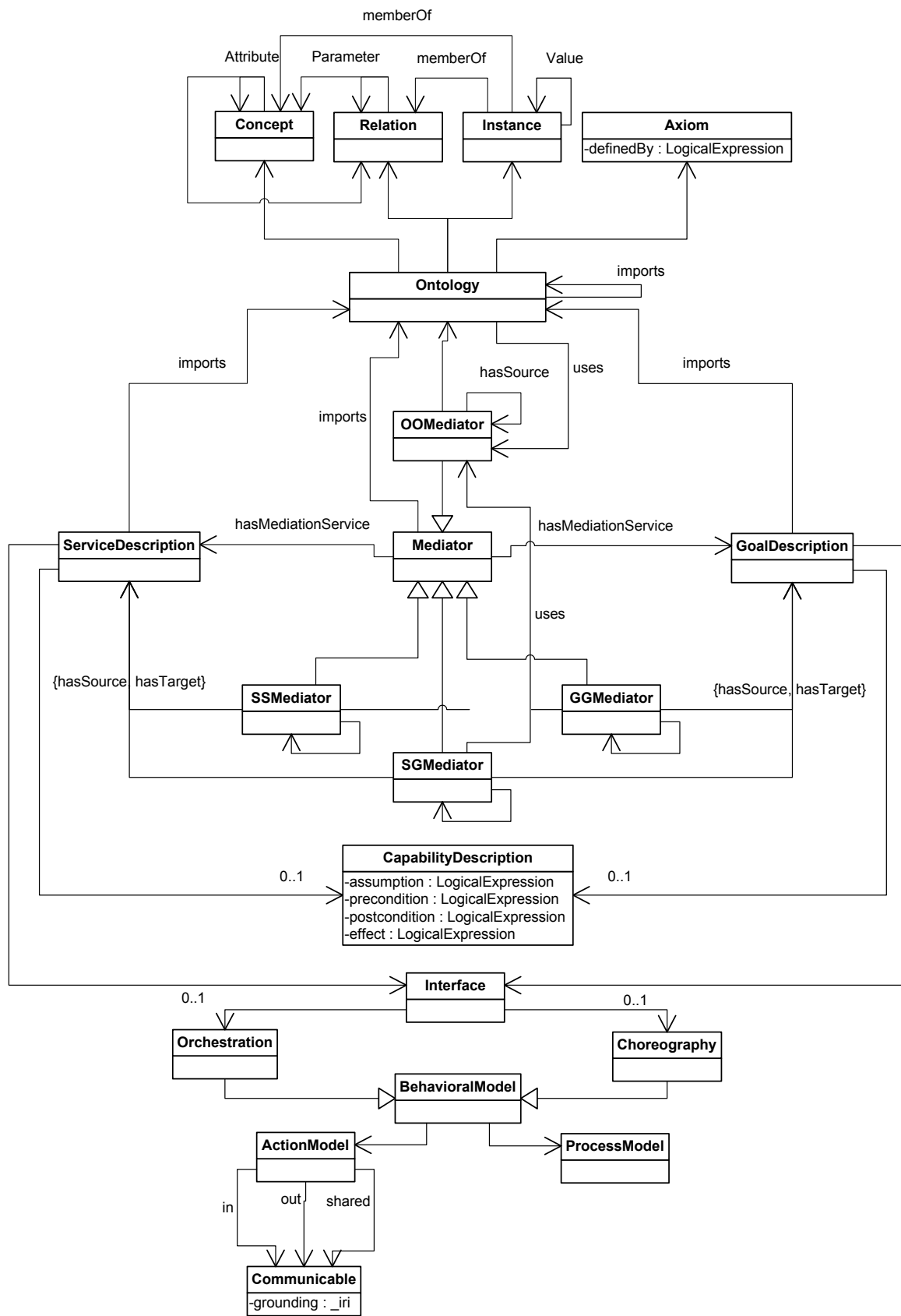
Figure C – OASIS Semantic SOA Reference Ontology
