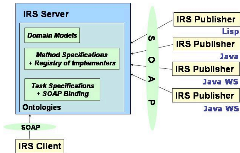
Figure 3. The Web Services Usage Scenario.
