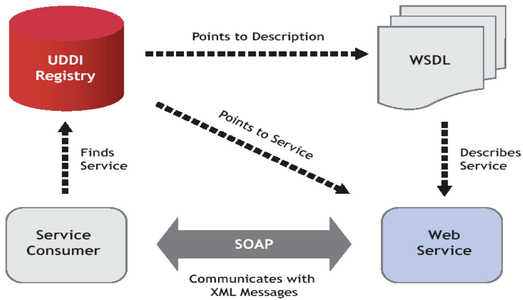
Figure 3. The Web Services Usage Scenario.
