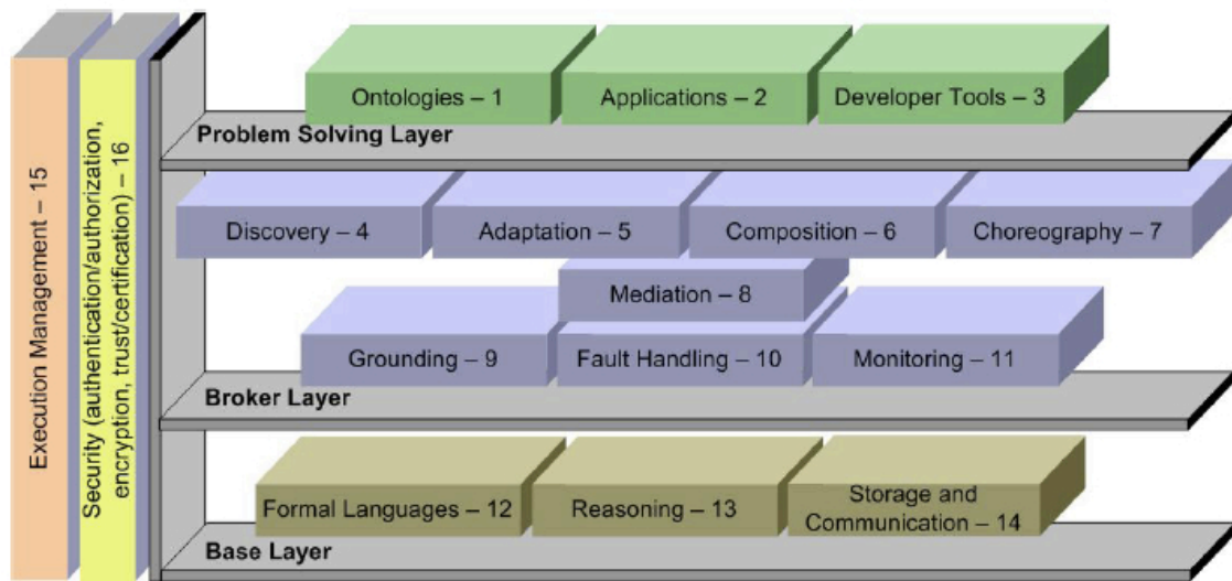
Figure 7. The Internal Architecture of a Semantic Execution Environment.
