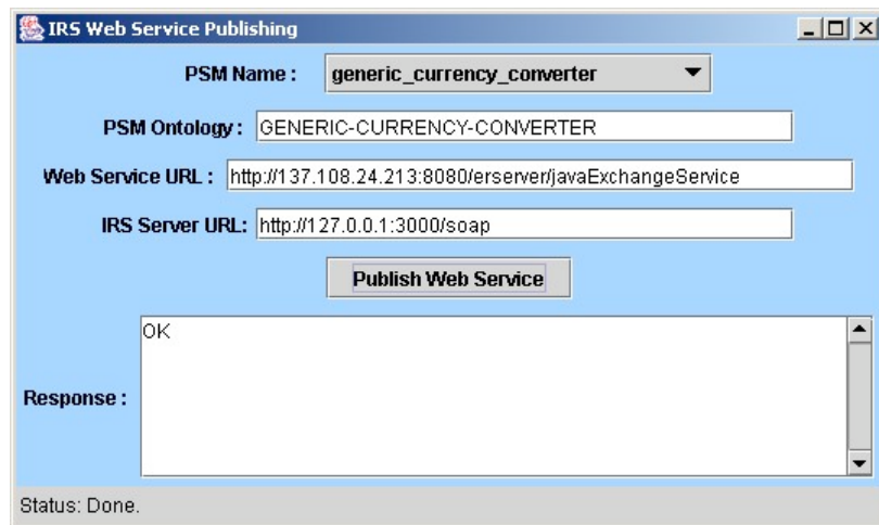
Figure 5. The Interface for the IRS-II Web Service Publisher.
