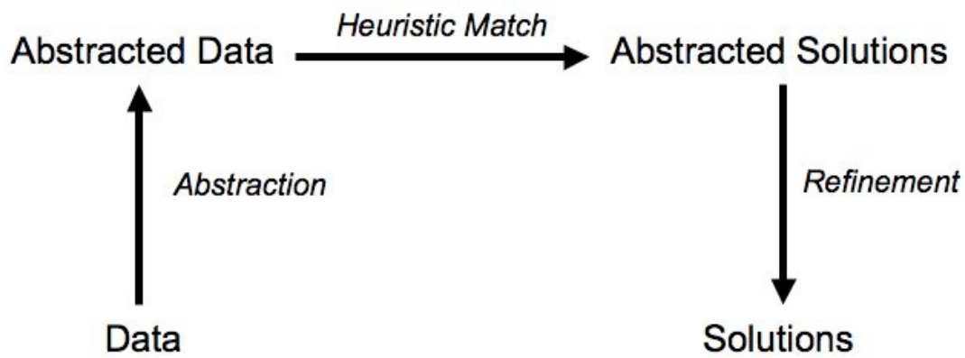
Figure 1. The Heuristic Classification PSM.
